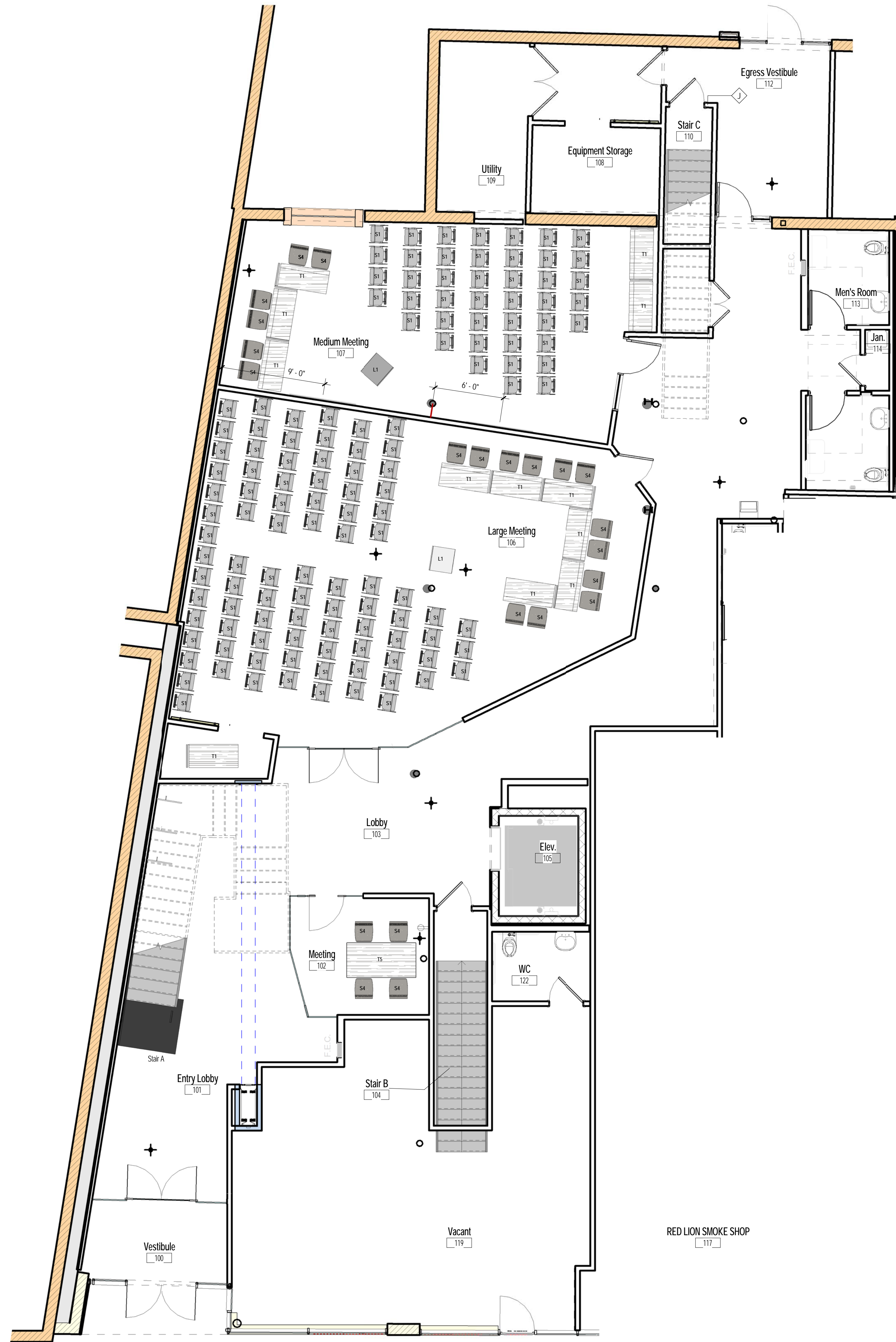
1 01 FIRST FLOOR - FURNITURE FURN-01 3/16" = 1'-0"
